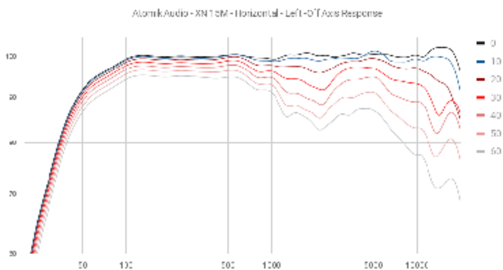
Horizontal - Left - Off Axis Response
