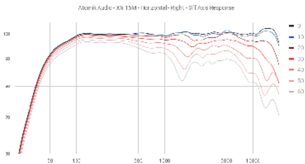
Horizontal - Right - Off Axis Response
