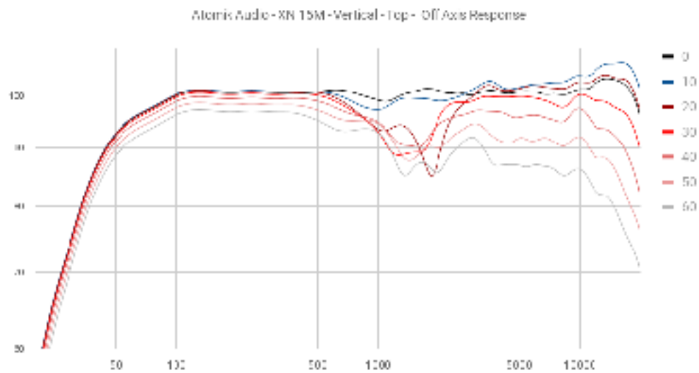
Vertical - Top - Off Axis Response
