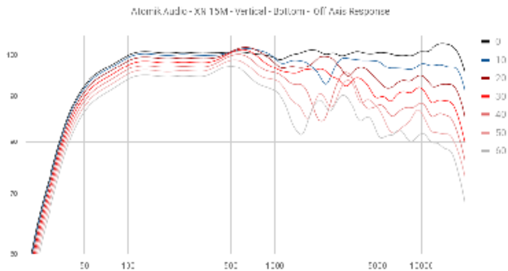
Vertical - Bottom - Off Axis Response
